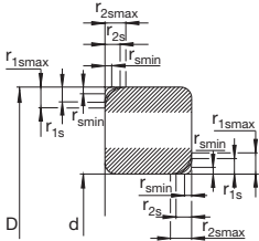
Radiallager
