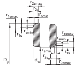
Axiallager
