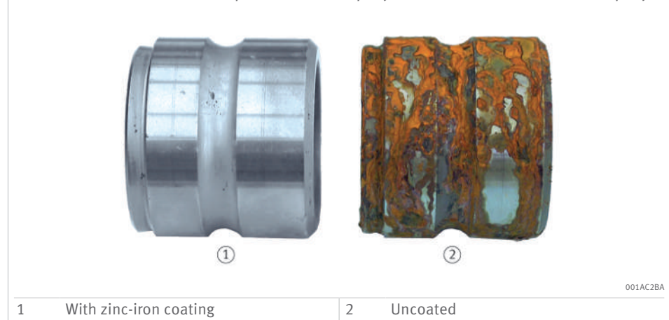
3 Coated and uncoated part after salt spray test, test time 24 h in salt spray
