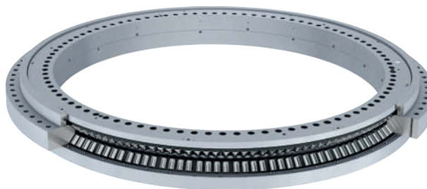
15 Tapered roller bearing system for wind turbines, coated with Corrotect H on all outside surfaces
