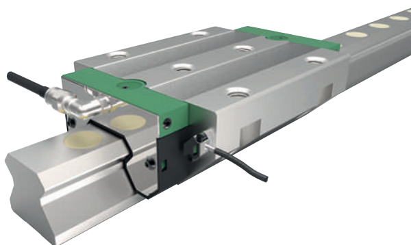
24 Linear recirculating roller bearing and guideway assembly RUE, coated with Durotect CK on the outer surfaces
