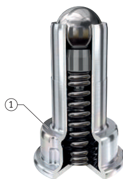
9 Selector rod detent pin from manual transmission
