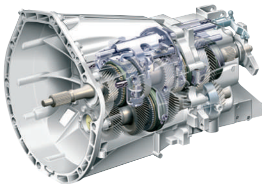
10 Application example, manual transmission
