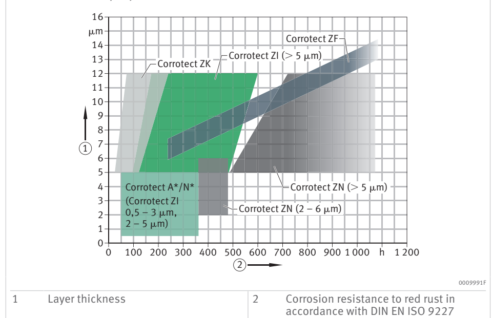
2 Comparison of Corrotect coating systems (cathodic corrosion protection) in the neutral salt spray test
